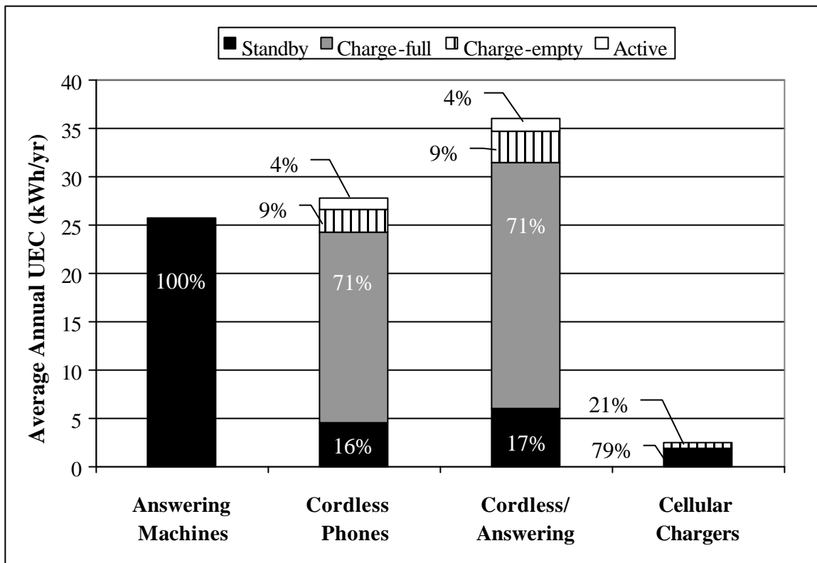
Figure 4-2. Mode Contributions to UEC Values for Telephony Products
